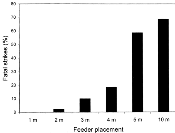
FIG. 1. The proportion of bird fatalities (%) at windows increases as bird feeders are placed farther from the glass surface. Data are from field experiments at Germansville, Lehigh County, Pennsylvania, 1991–1992.
